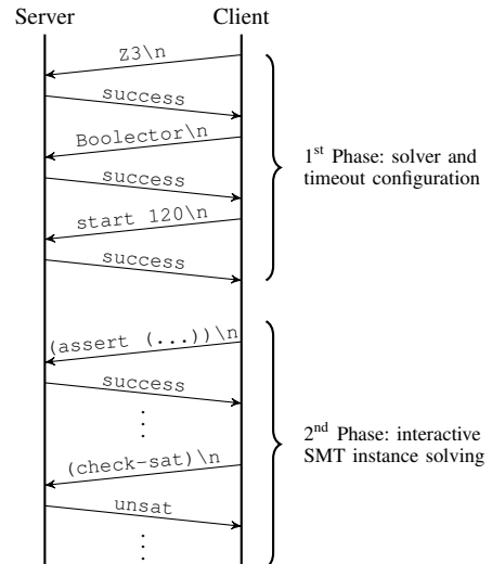
Fig. 5. Example communication between server and client
