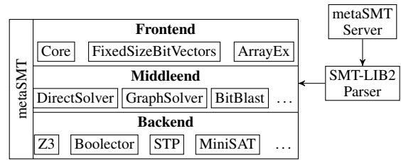
Fig. 2. metaSMT Architecture
